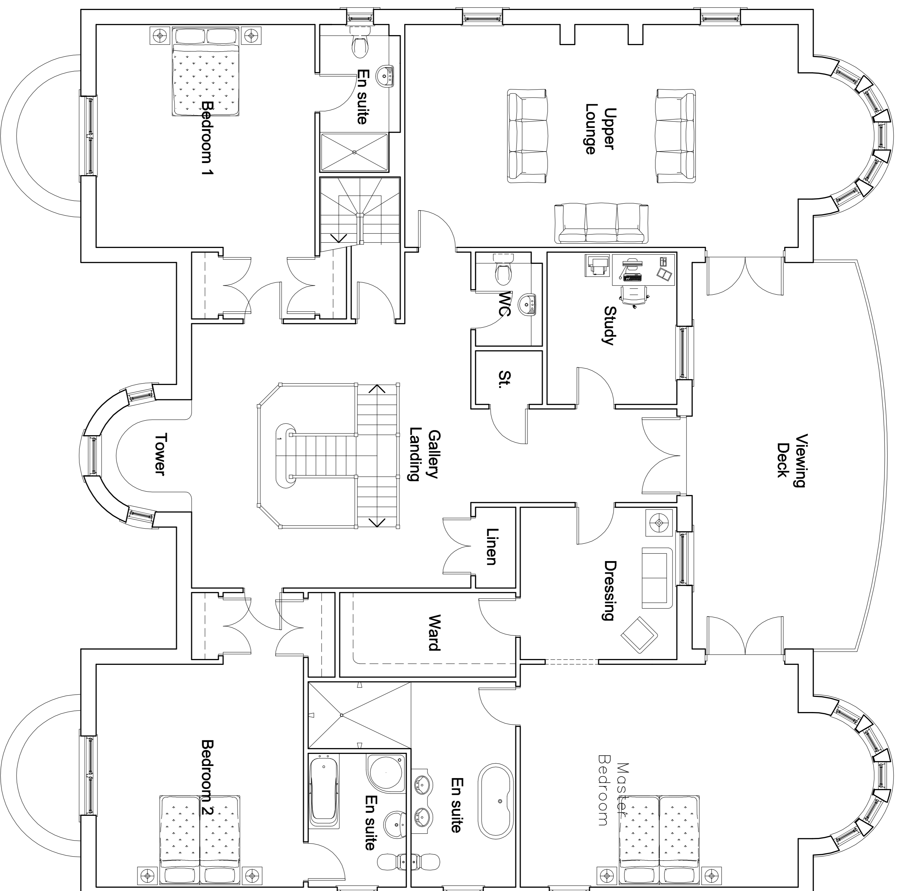
First Floor Plan (GIFA 265 sq.m)
